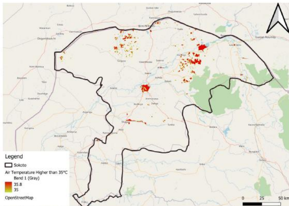
Figure 3. Areas at risk under the SSP 2-4,5 scenario
